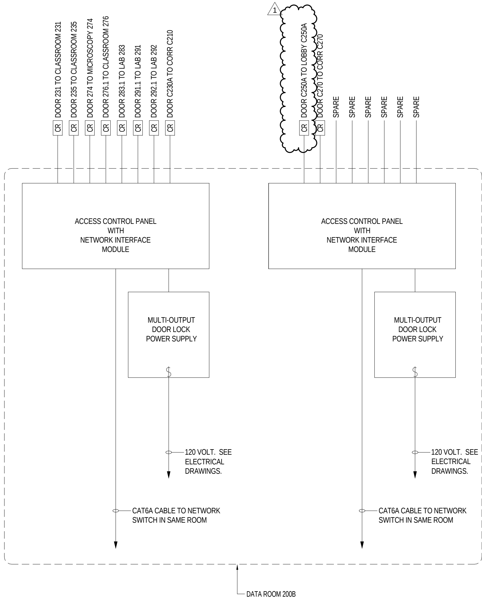
ACCESS CONTROL SYSTEM DIAGRAM-LEVEL 2 SCALE: NONE
