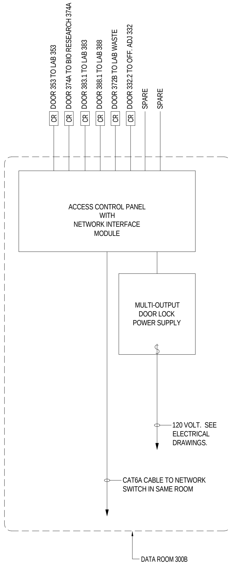
ACCESS CONTROL SYSTEM DIAGRAM-LEVEL 3 SCALE: NONE
